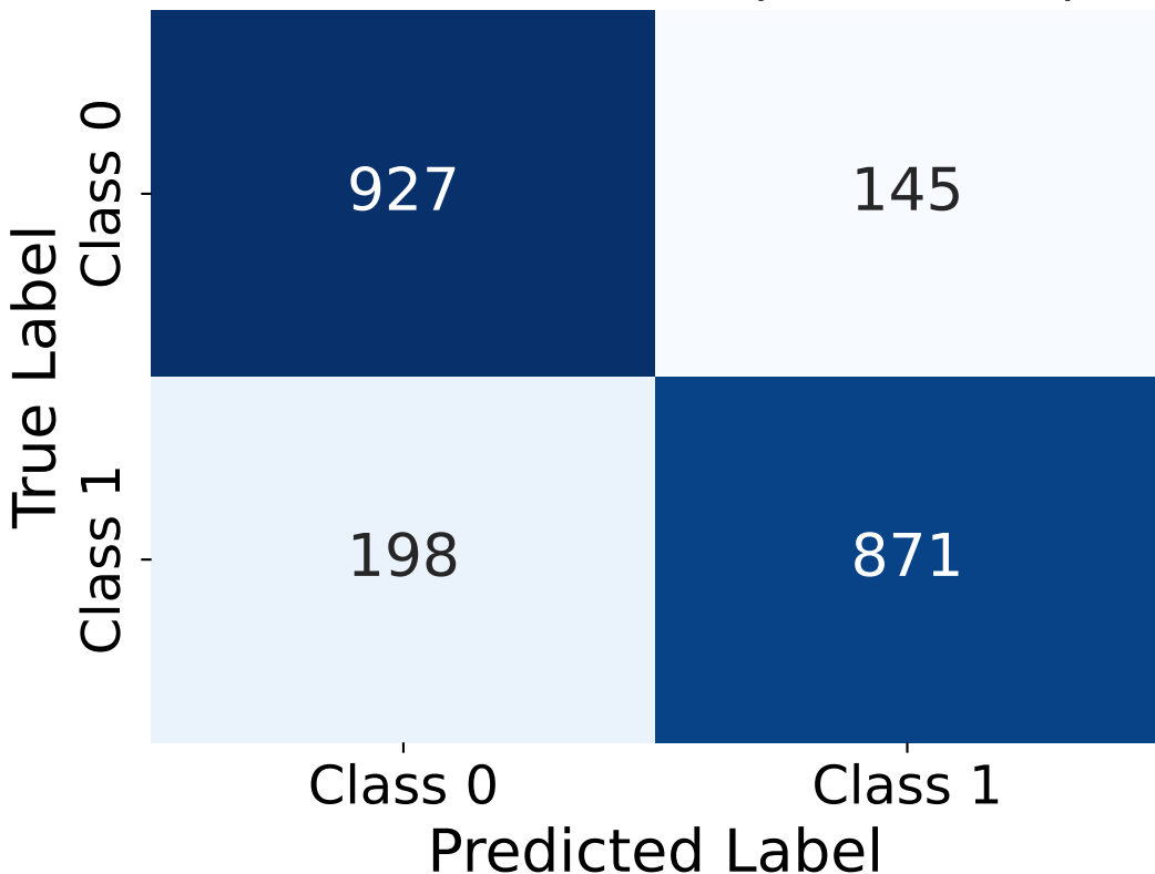
Confusion Matrix (Validation)
